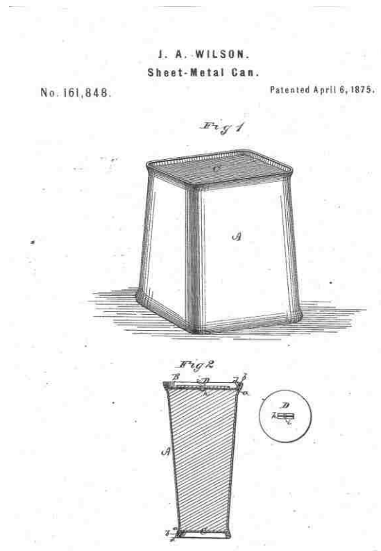
Figure 3.2 - Wilson's Tapered can. Taken from U. S. Patent 161,848, April 6, 1875.
