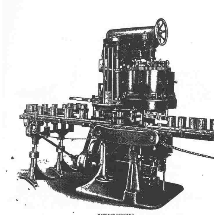
Figure 3.8 - Max Ams No. 498 Double Seamer. Max Ams Machine Company, Catalogue No. 17 - Panama Exposition, 3.
